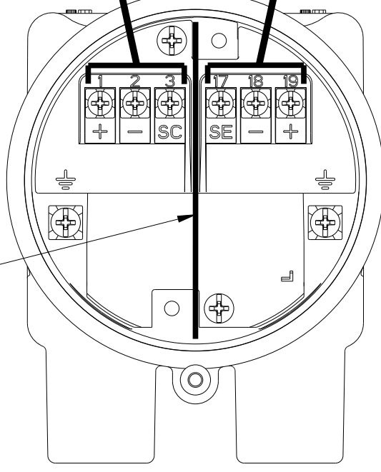
8750WDMR/W FLOWTUBE REMOTE JUNCTION BOX
