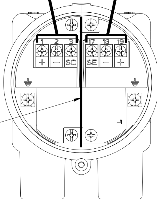
8750WDMR/W FLOWTUBE REMOTE JUNCTION BOX
