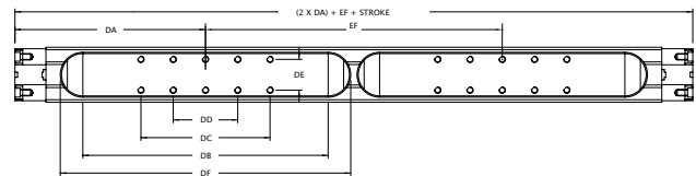
S1 Double Long Carriage Dimensions
