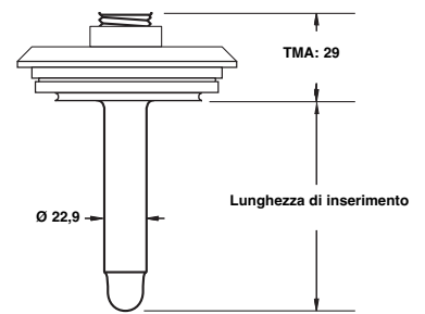
Varivent®
