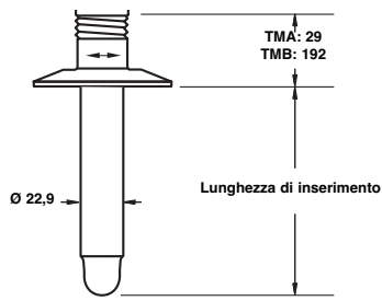
Tri-Clamp®
